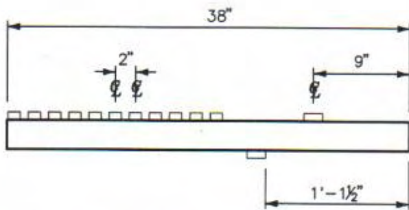
BACK LEG AND SLATS
