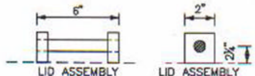
HANDLE ASSEMBLY
